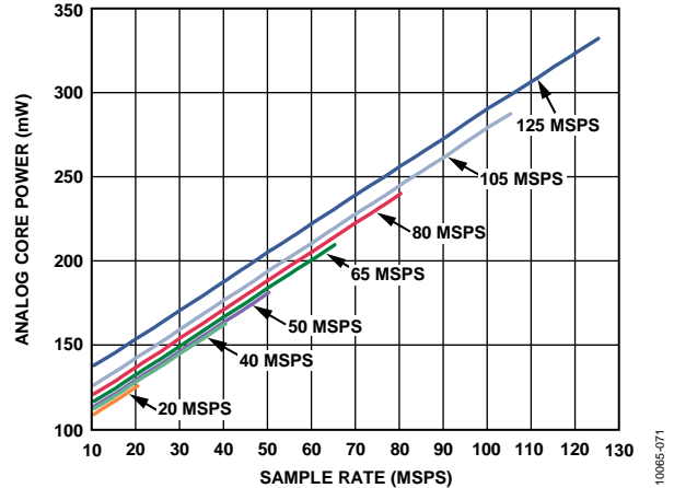
Figure 69. Analog Core Power vs. f_{SAMPLE} for f_{IN} = 10.3 \text{ MHz}
