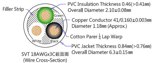
SVT 18AWGx3C截面圖 (Wire Cross-Section)
