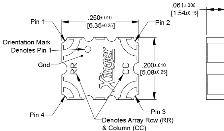
Dimensions are in Inches [Millimeters] XEC24P3-30G Mechanical Outline
