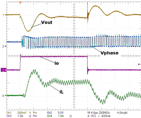
FIGURE 13. TRANSIENT LOAD TEST (PFM & PWM V_{IN} = 3.6V ; V_O = 1.6V ; I_O = 0A-1A )
