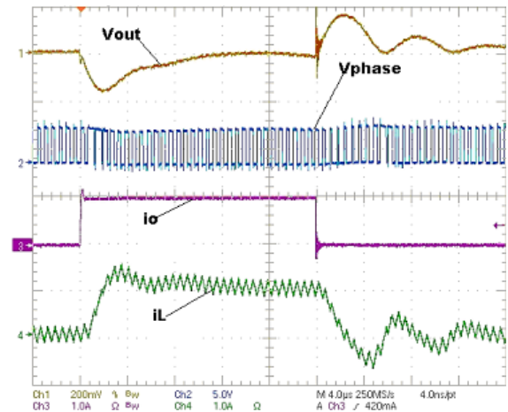
FIGURE 14. LOAD TRANSIENT IN PWM MODE ( V_{IN} = 3.6V ; V_O = 1.6V ; I_O = 0A-1A )
