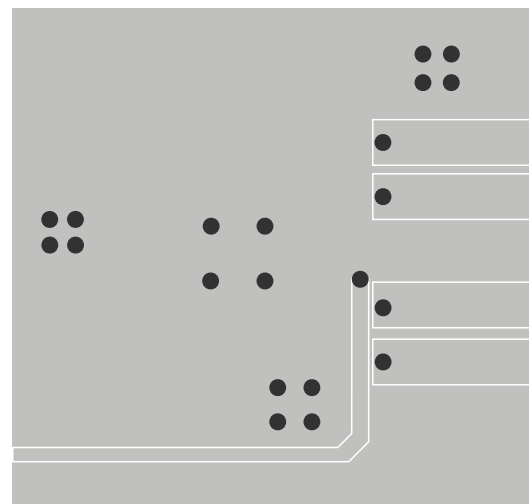
Figure 4 — Layer 2
