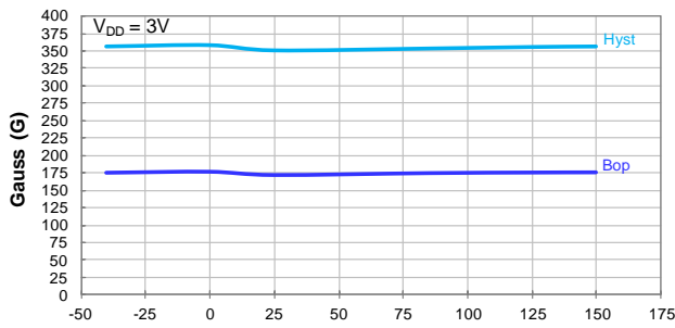
Temperature (°C) Switch Operate Point Bop vs Temperature
