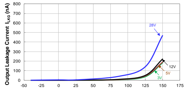
Temperature ( ^\circ\text{C} ) Output Leakage Current vs Temperature
