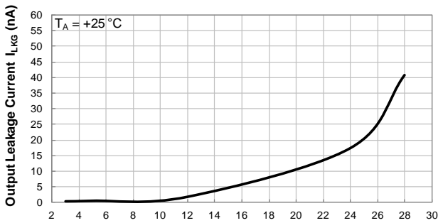
Supply Voltage (V) Output Leakage Current vs Supply Voltage
