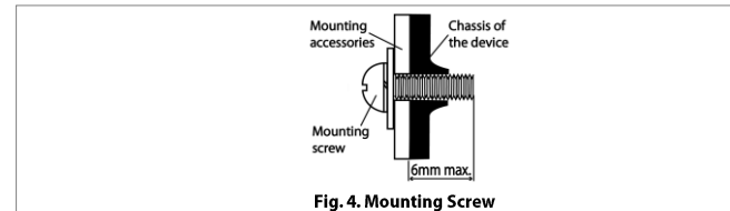
Fig. 4. Mounting Screw
