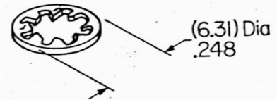
AT081E Star Washer S200, SB21, SB265
