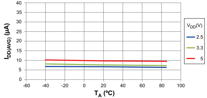
Average Supply Current vs. Ambient Temperature
