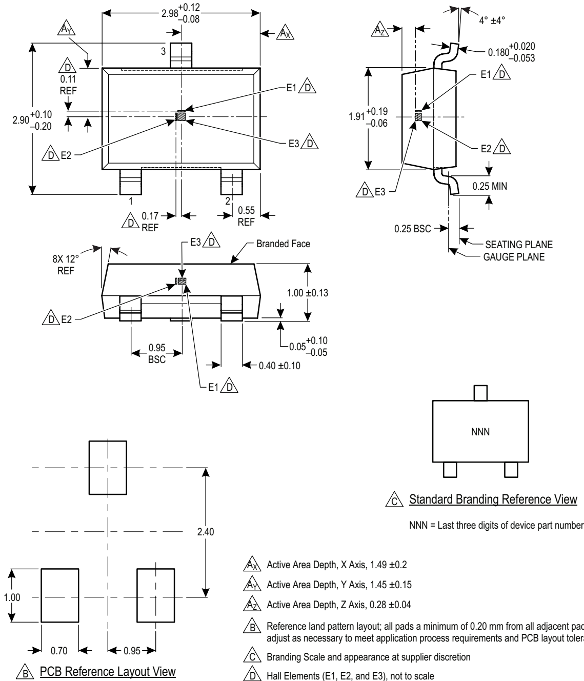
Figure 8: Package LH, 3-Pin SOT23-W
