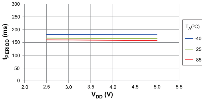
Average Period vs. Supply Voltage
